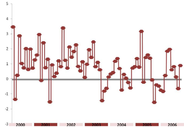
Difference in Maximum Temperatures from Historical Record, GASN station (Diouana)
