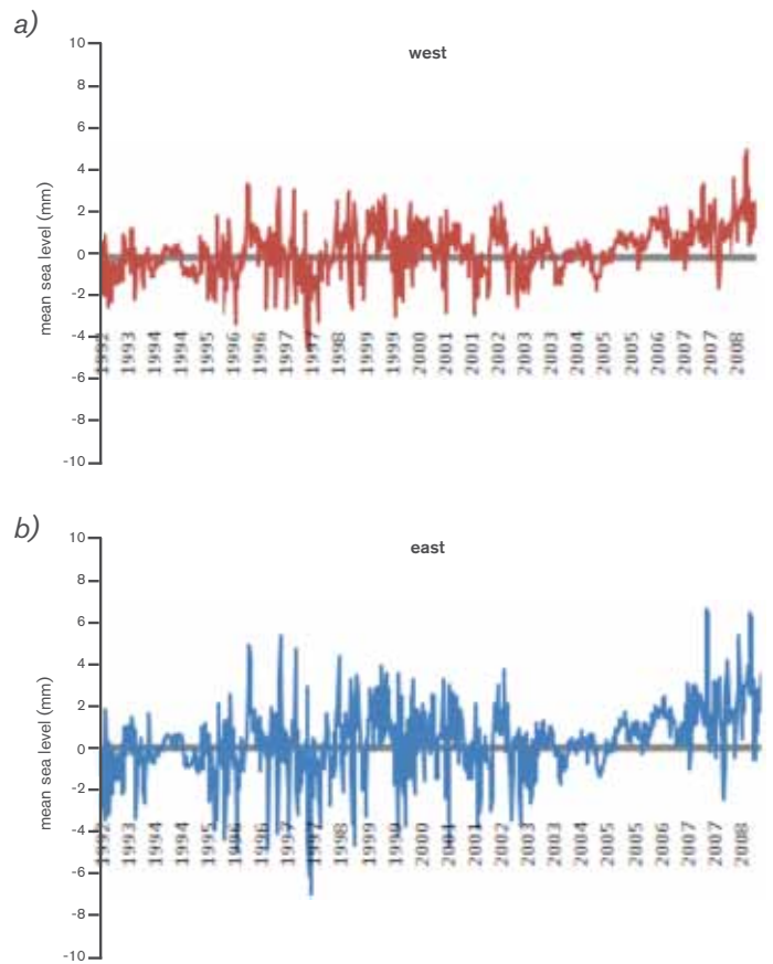
Figure 15. SSH time series from satellite altimetry.
