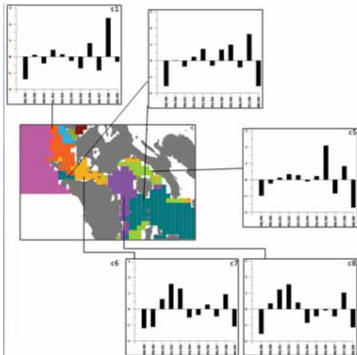
Figure 40. Anomaly signals for the NE monsoon (Dec-Feb) in surface chl (mg/m³).
