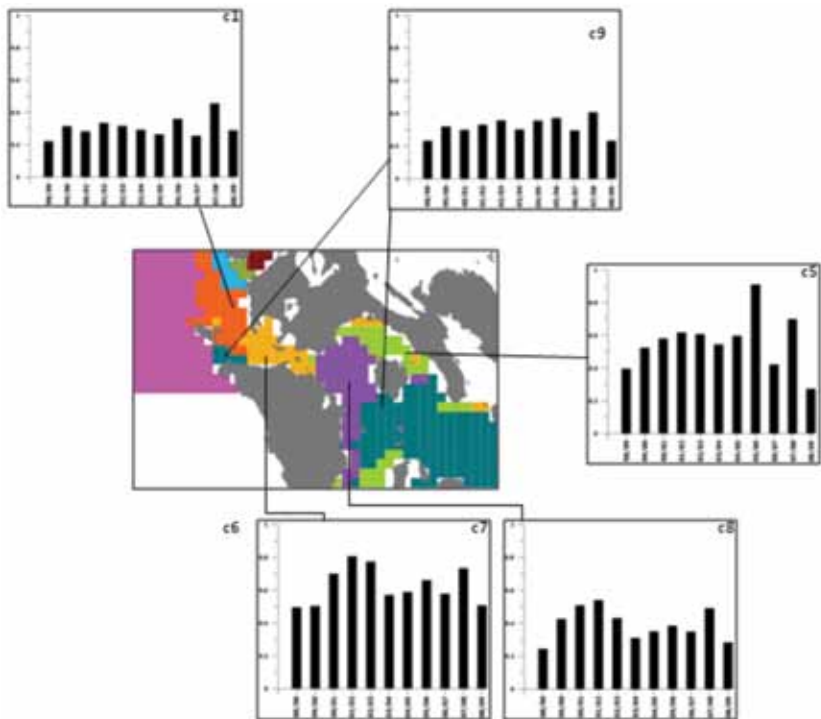
Figure 39. Average signal during the NE monsoon (Dec-Feb) in surface chl (mg/m³). Values are standardized (normalized by mean and st dev) for comparison (Dec 1997-Feb 2009).
