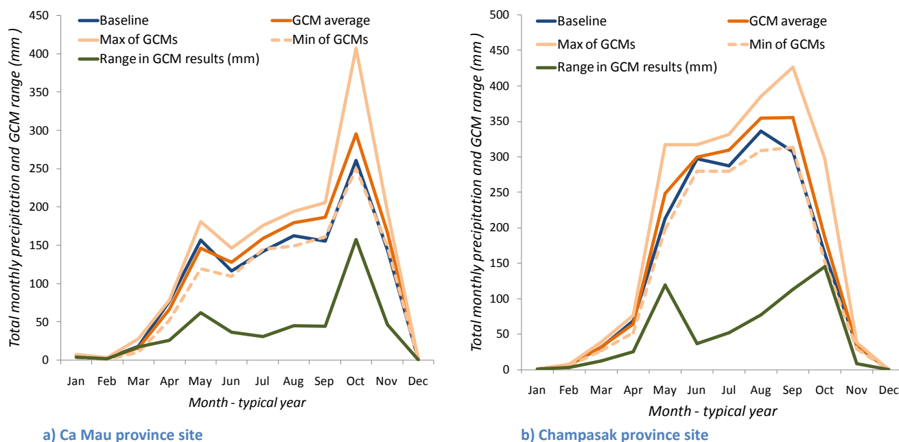
Figure 4-9: Intra-annual comparison of the range in GCM precipitation: results for a) Ca Mau and b) Champasak provinces
