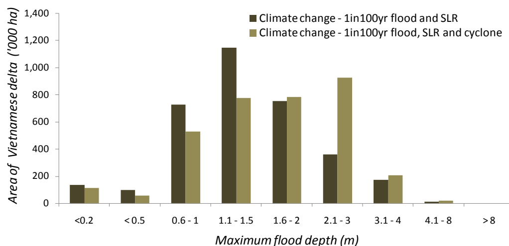
Figure 4-27: Comparison of maximum flood depth for climate change scenarios with and without cyclone impacts
