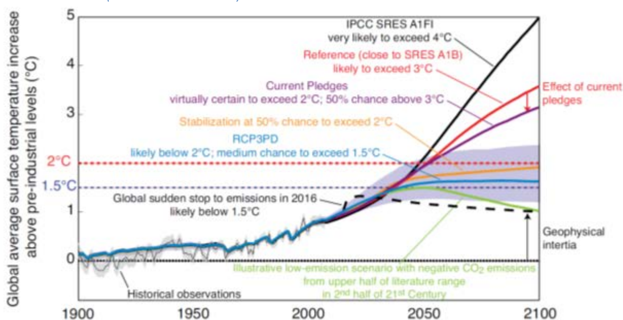
Figure 3-11: Projected changes in global mean surface temperatures using high (A1F1), moderate (A1B), and low (RCP3-PD) emissions scenarios (Source: World Bank 2012)
