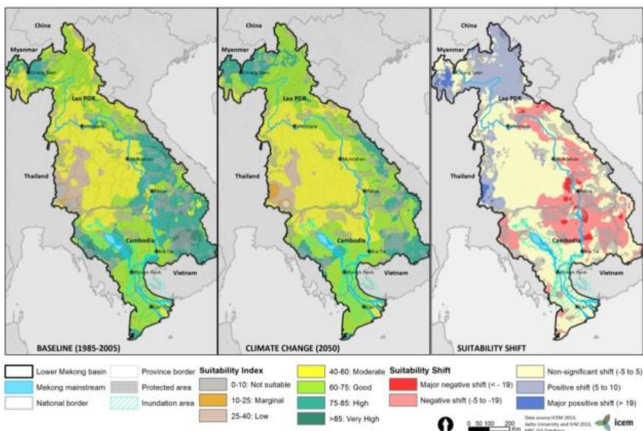
Figure 5-2: Rubber suitability in the Lower Mekong Basin - results of LUSET modeling
