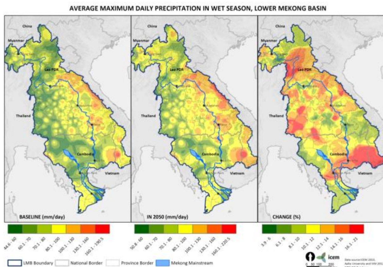
Figure 4-24: Projected increases in peak daily precipitation for the LMB
