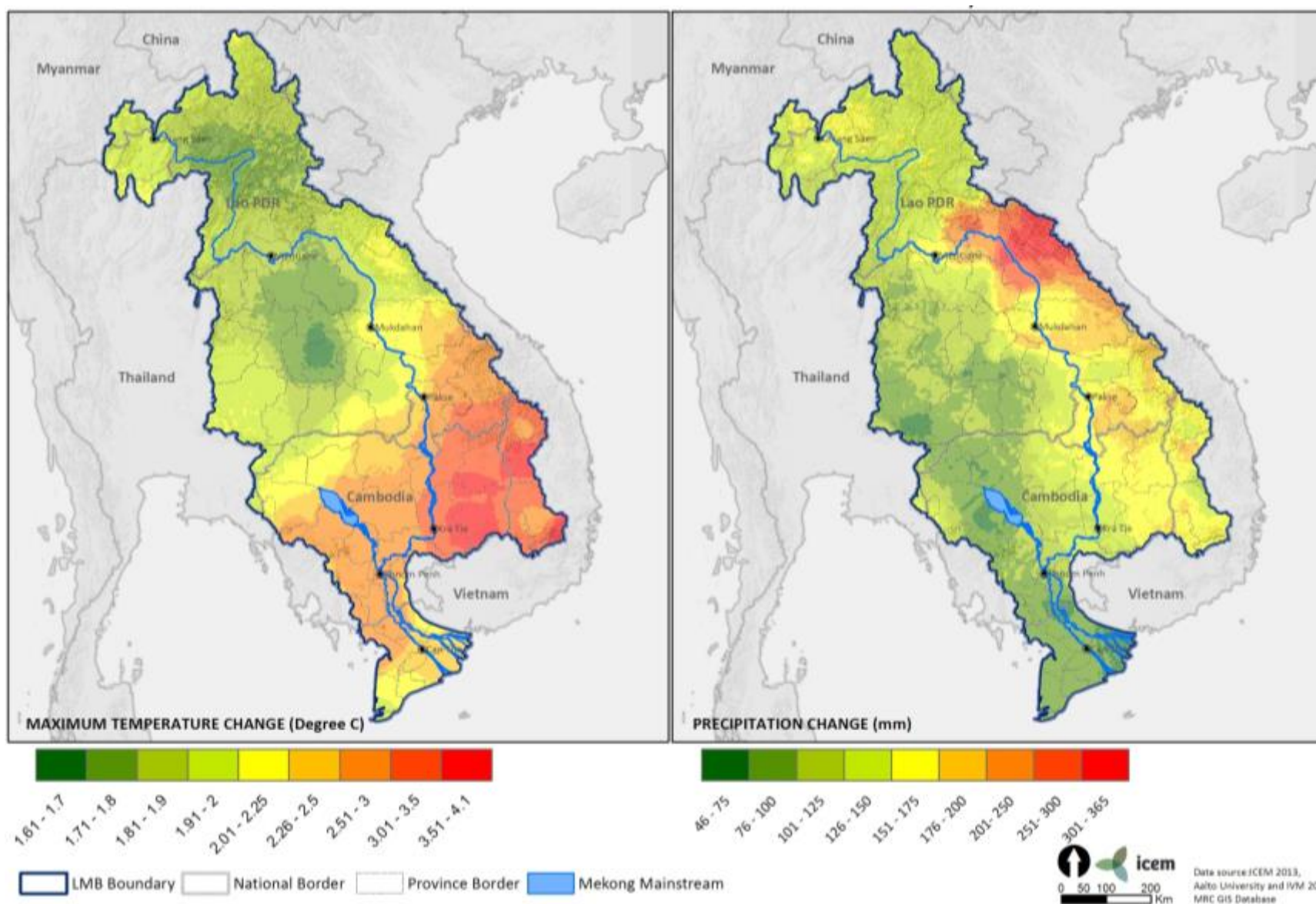
Figure 4-17: Projected annual precipitation and annual average maximum daily temperature changes in the Lower Mekong Basin
