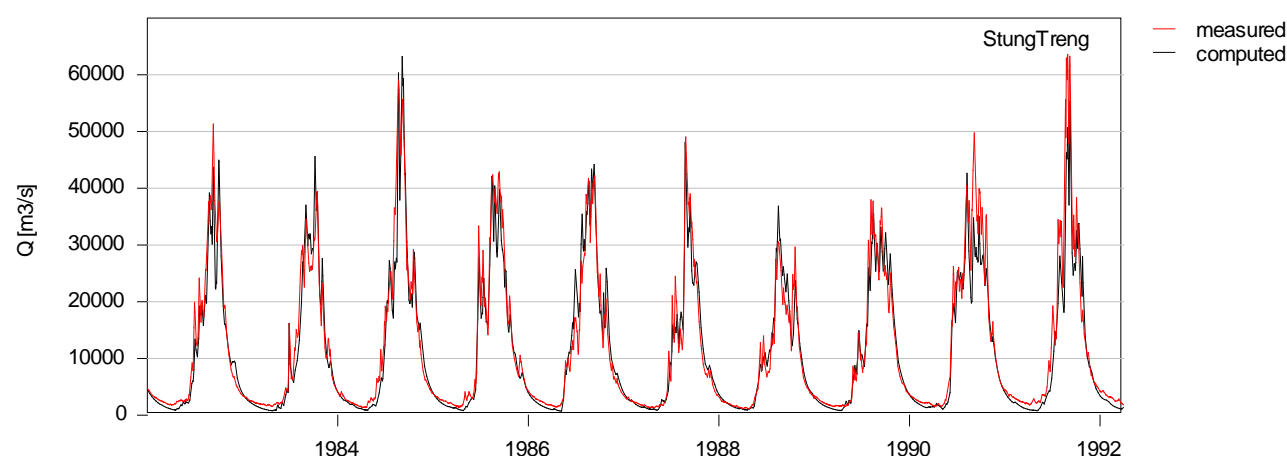
Figure 3-16: Observed (red line) and computed (black line) daily flows at Stung Treng station (Lauri 2011)
