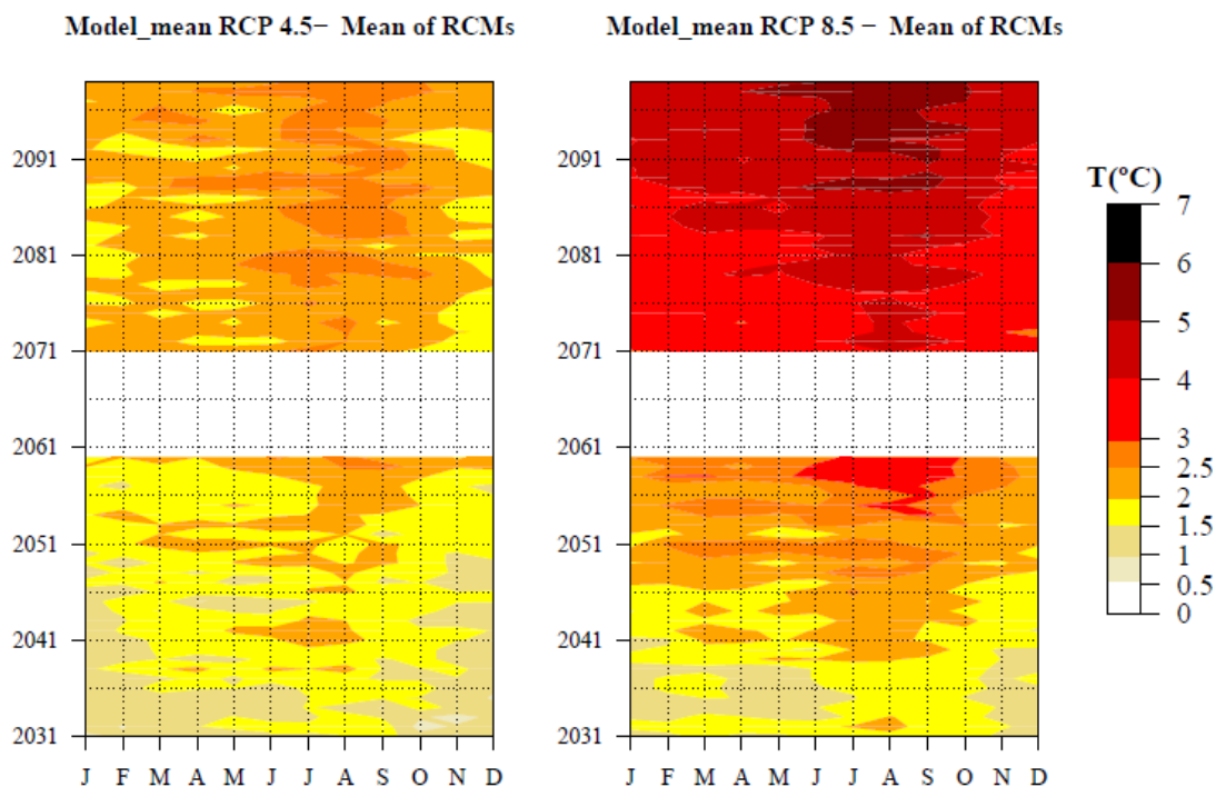
Figure 9: Projected monthly air temperature anomalies to 1970-1999
