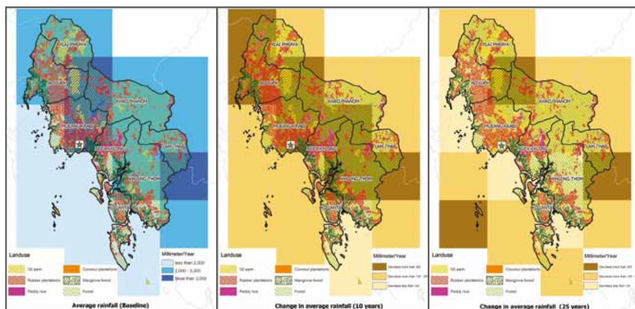
Figure 7: Changes in average annual rainfall over Krabi province: 1980s, 2015-2024 and 2030s
