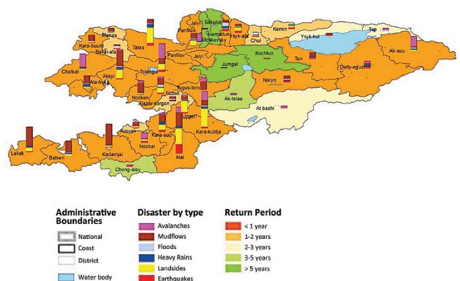
FIGURE 12 Expected trends of climate related hazards in Kyrgyz Republic
