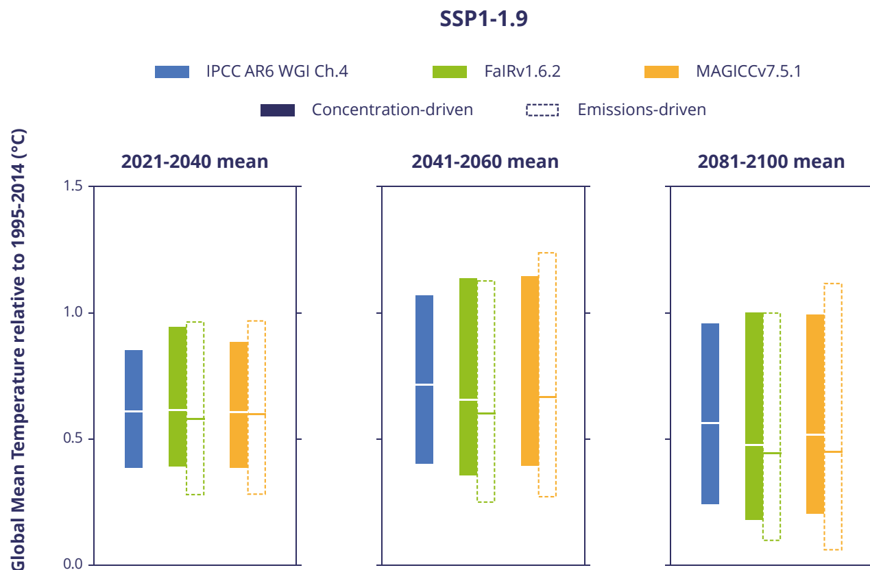
FIGURE 5: Comparison of 21 st century global mean temperature change for concentration- and emissions-driven emulator runs under the same very low emissions scenario (SSP1-1.9). Central estimates and very likely (5-95% model) ranges are provided for the near-term (2021-2040), mid-term (2041-2060), and long-term (2081-2100) relative to the recent reference period 1995-2014. The IPCC AR6 WGI Chapter 4 assessment as well as concentration-driven estimates shown in darker shading, emissions-driven estimates in lighter shading. Figure based on IPCC AR6 WGI Cross-Chapter Box 7.1 Figure 1.
