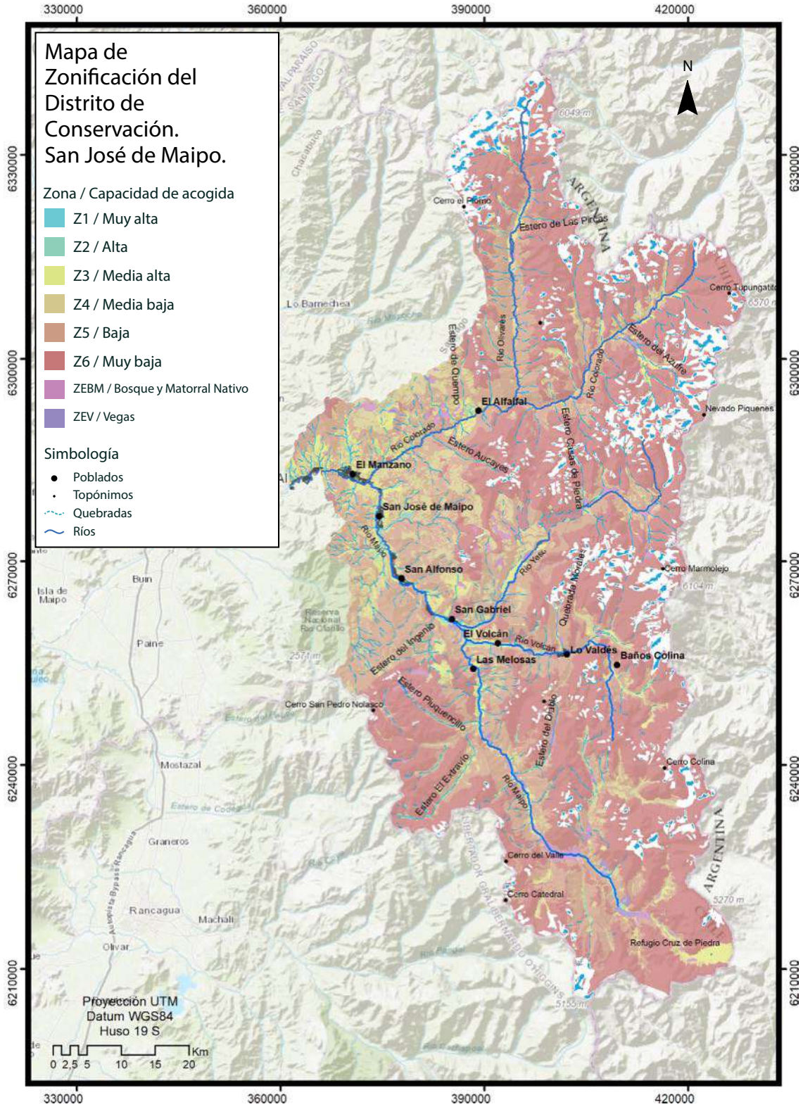
Map 3: Zoning of the San José de Maipo Conservation District, Chile. (Source: GEF Montaña)
